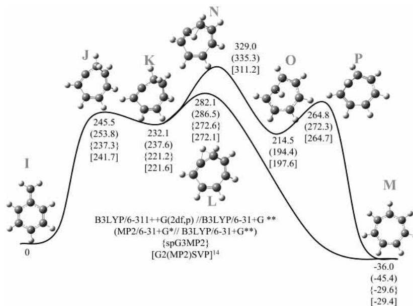
Figure 10. Calculated potential energy profiles for the isomerization of the benzylum cation to the tropylium cation; see the text.
