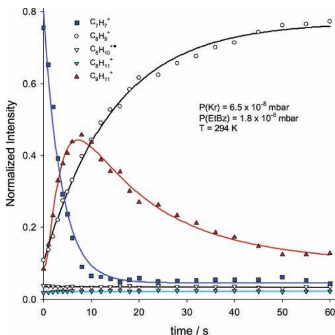
Figure 5. Plot of normalized intensity vs time for the reaction of the \text{Bz}^+ fraction of the m/z 91 signal with neutral EtBz. This kinetics plot corresponds to the mass spectra in Figure 4.
