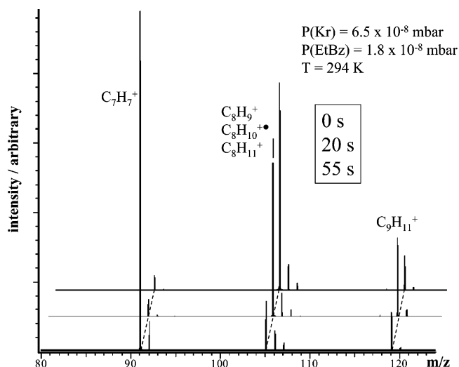
Figure 4. Mass spectra recorded after no delay as well as after 20- and 55-s delays following the isolation of ions at m/z 91, 105, 106, 107, 119, and 120. These delays followed the 4-s reaction of \text{Kr}^+ with neutral EtBz.
